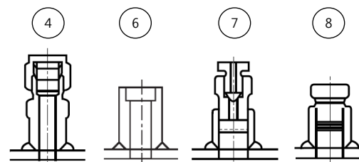
END CONNECTORS
